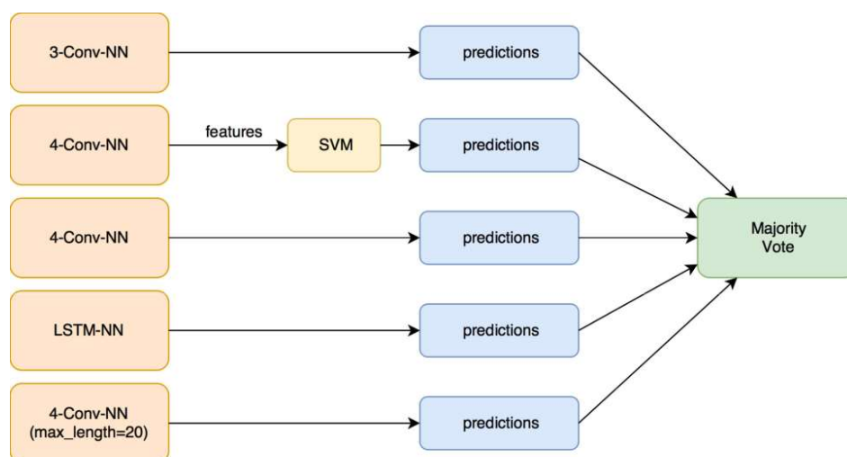
Figure 10: Flowchart of Majority Voting Ensemble.
